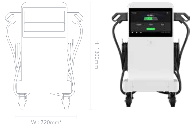
MAXICHARGER DC COMPACT PEDESTAL FRONT VIEW
