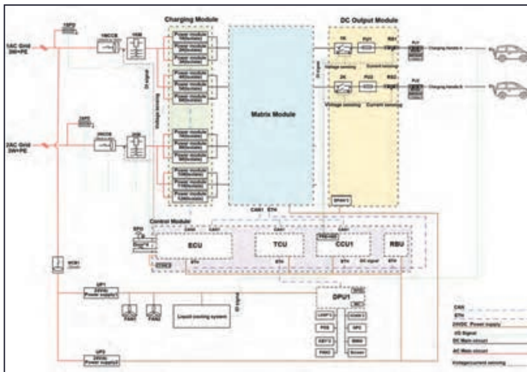
Figure 3-13 Electrical Diagram (Liquid-cooled Model)
