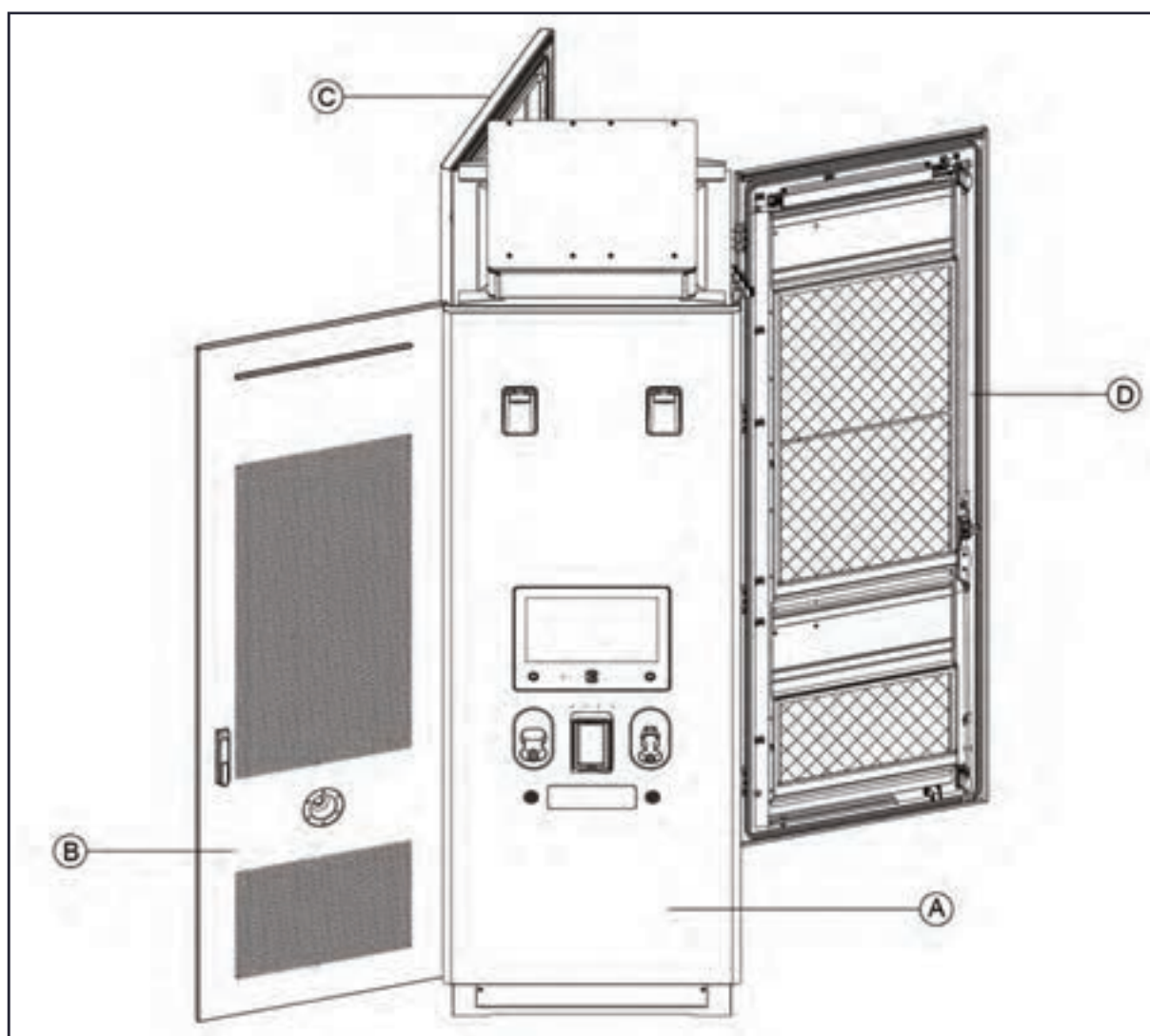
Figure 3-3 Four Doors of the Charging Station
