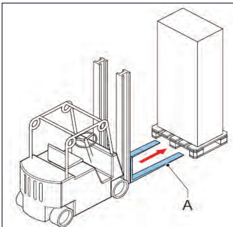
Figure 4-39 Transporting the Cabinet by Forklift Truck
