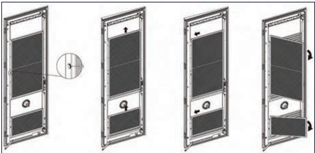
Figure 8-1 Removing the Air Inlet Filter
