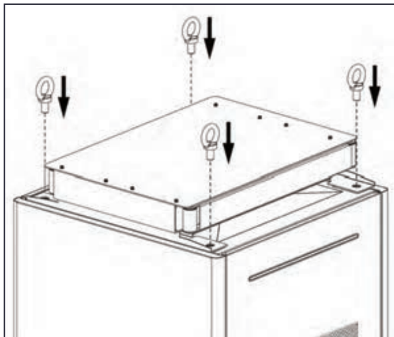
Figure 5-12 Installing the Eyebolts
