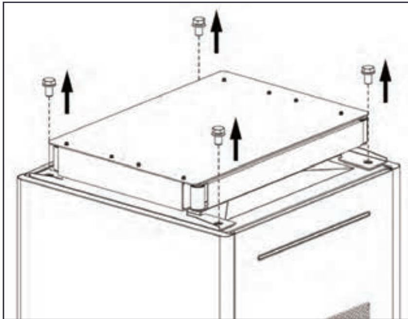
Figure 5-11 Removing the Screws
