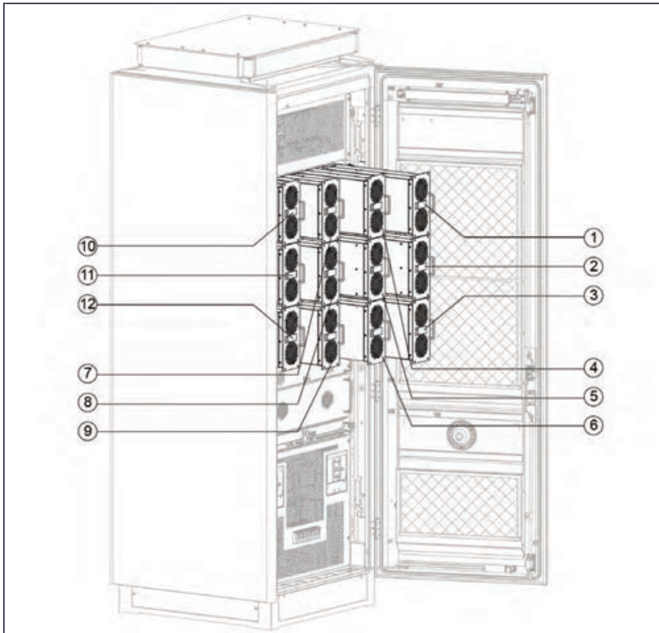
Figure 5-24 Charging Module Location
