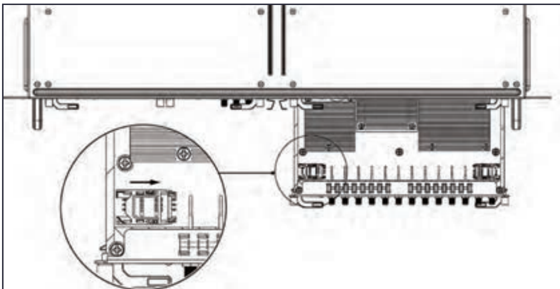
Figure 5-23 Opening the SIM Card Slot Cover
