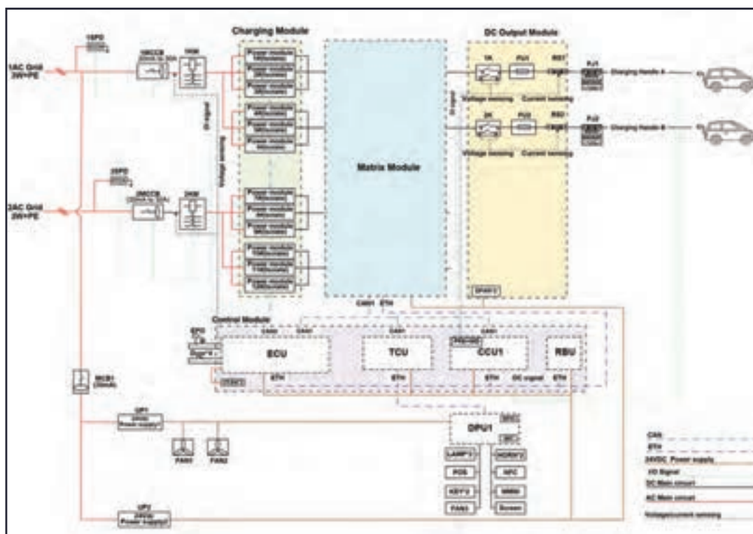
Figure 3-12 Electrical Diagram (Air-cooled Model)
