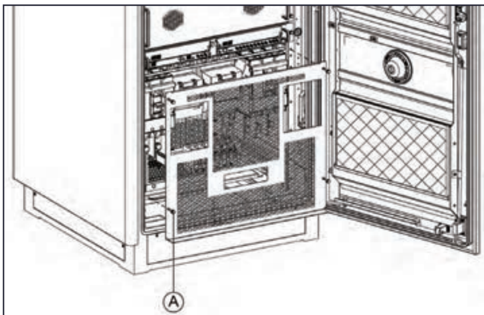
Figure 5-16 Removing the Cover Plate
