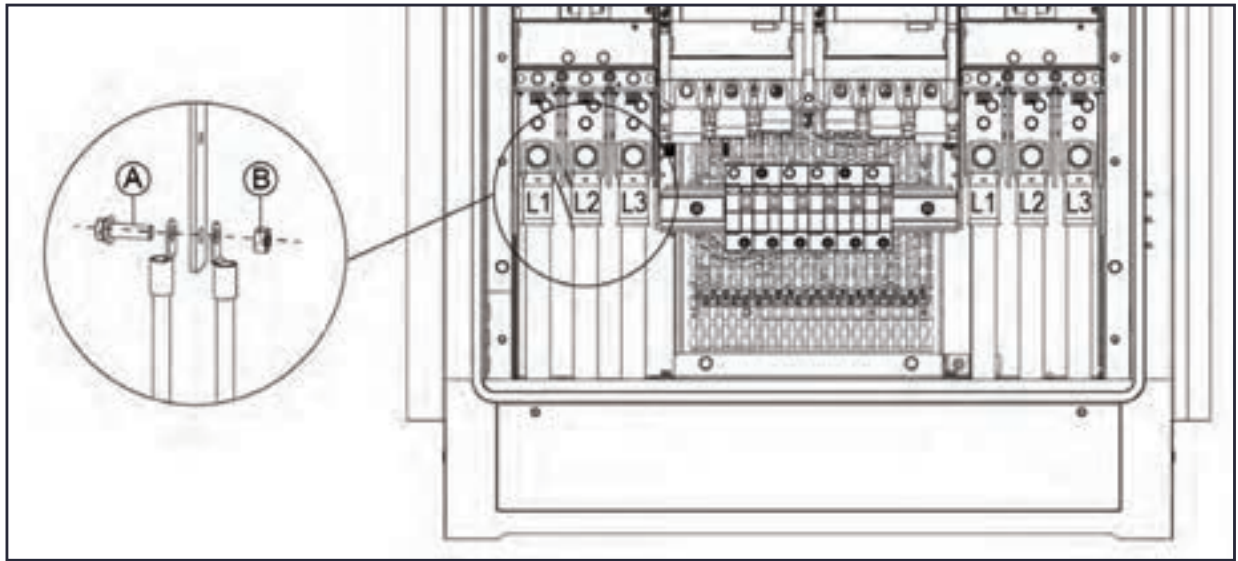
Figure 5-17 Connecting the AC Input Power Cables
