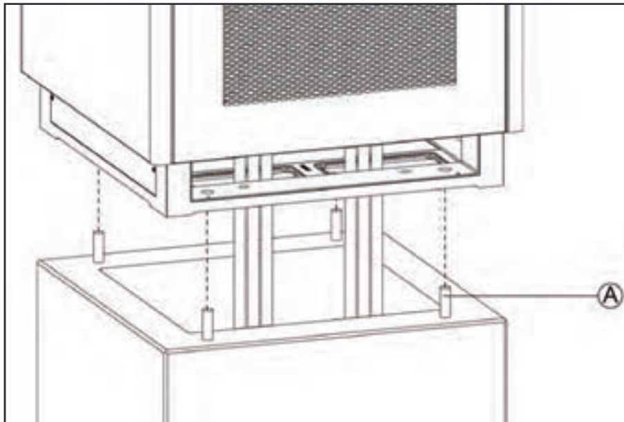
Figure 5-14 Lowering the Cabinet
