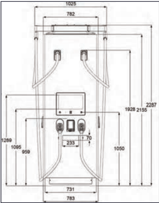
Figure 3-9 DH480 Dimensions (Front View)
