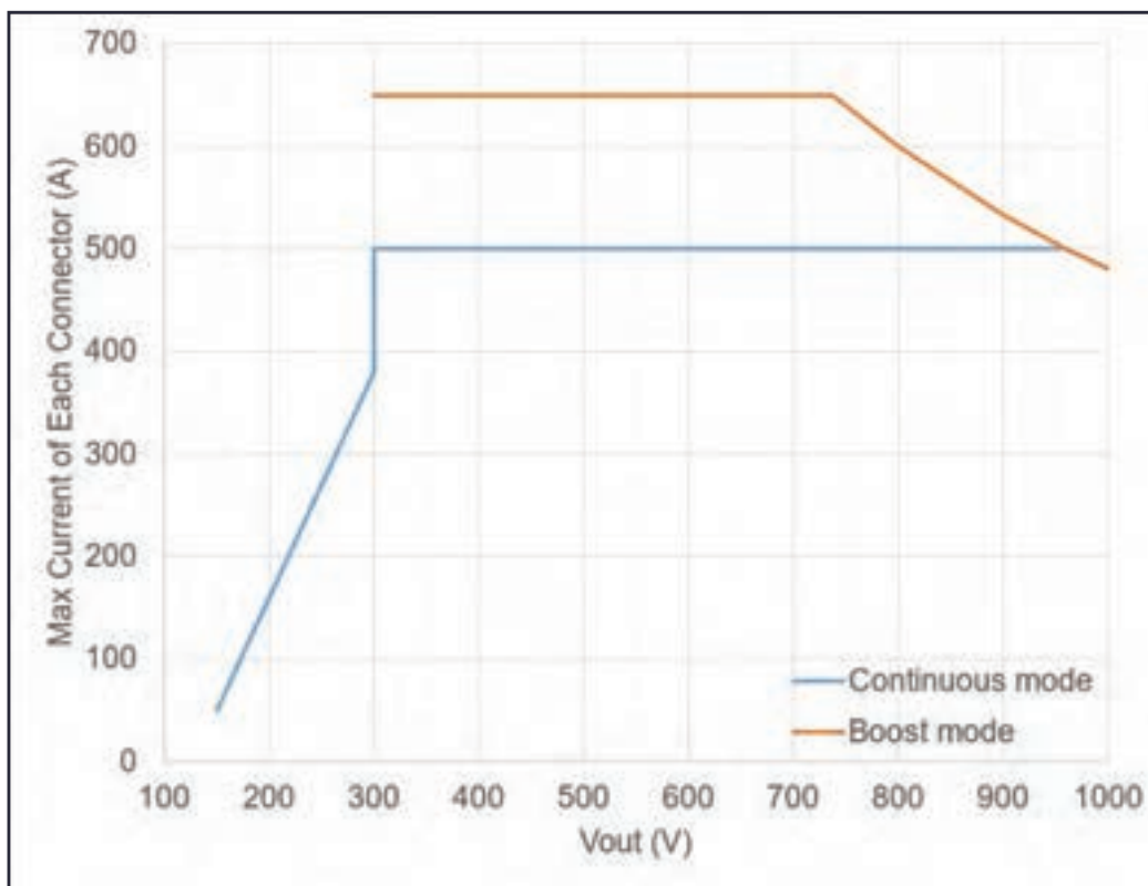
Figure 9-2 Output Voltage-Current Curve (Liquid-cooled)
