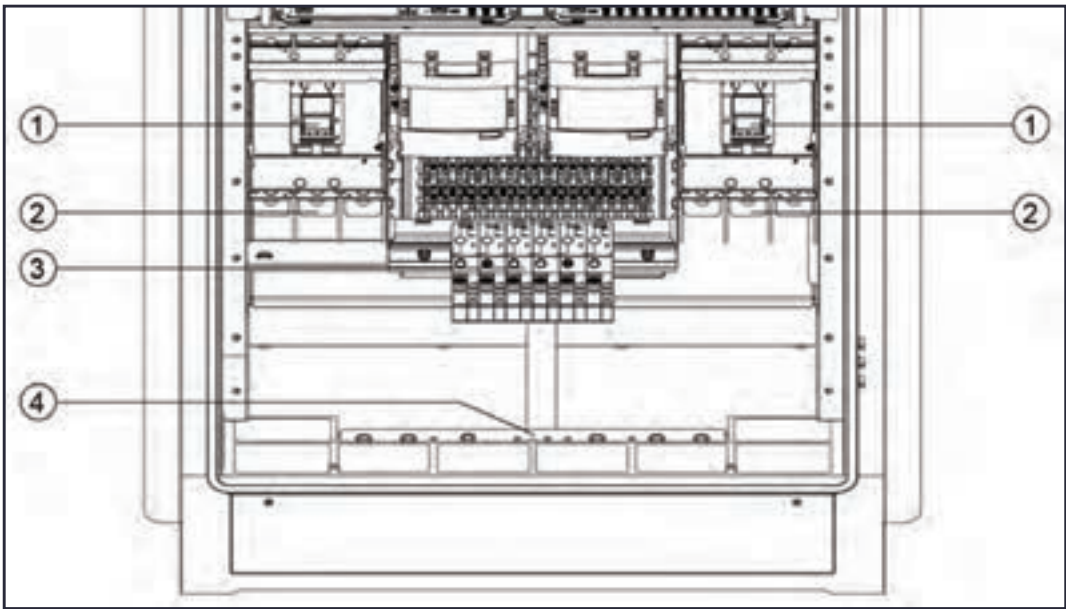
Figure 3-8 AC Input Unit (Inside)
