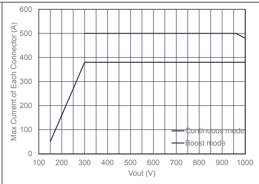
Figure 9-1 Output Voltage-Current Curve (Air-cooled)
