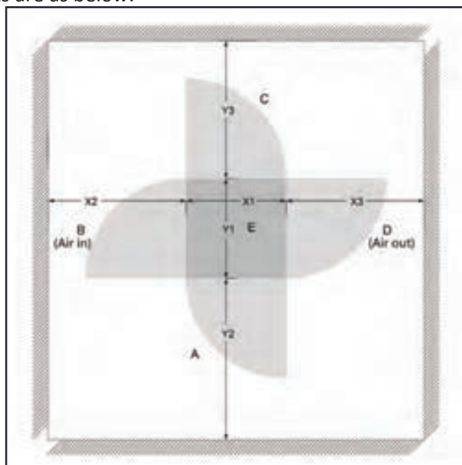
Figure 4-37 Space Requirements
