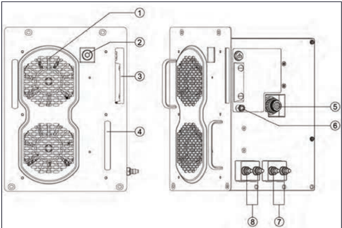
Figure 3-17 Cooling Unit
