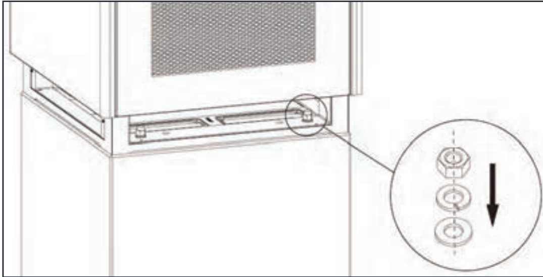
Figure 5-6 Securing the Cabinet onto Foundation
