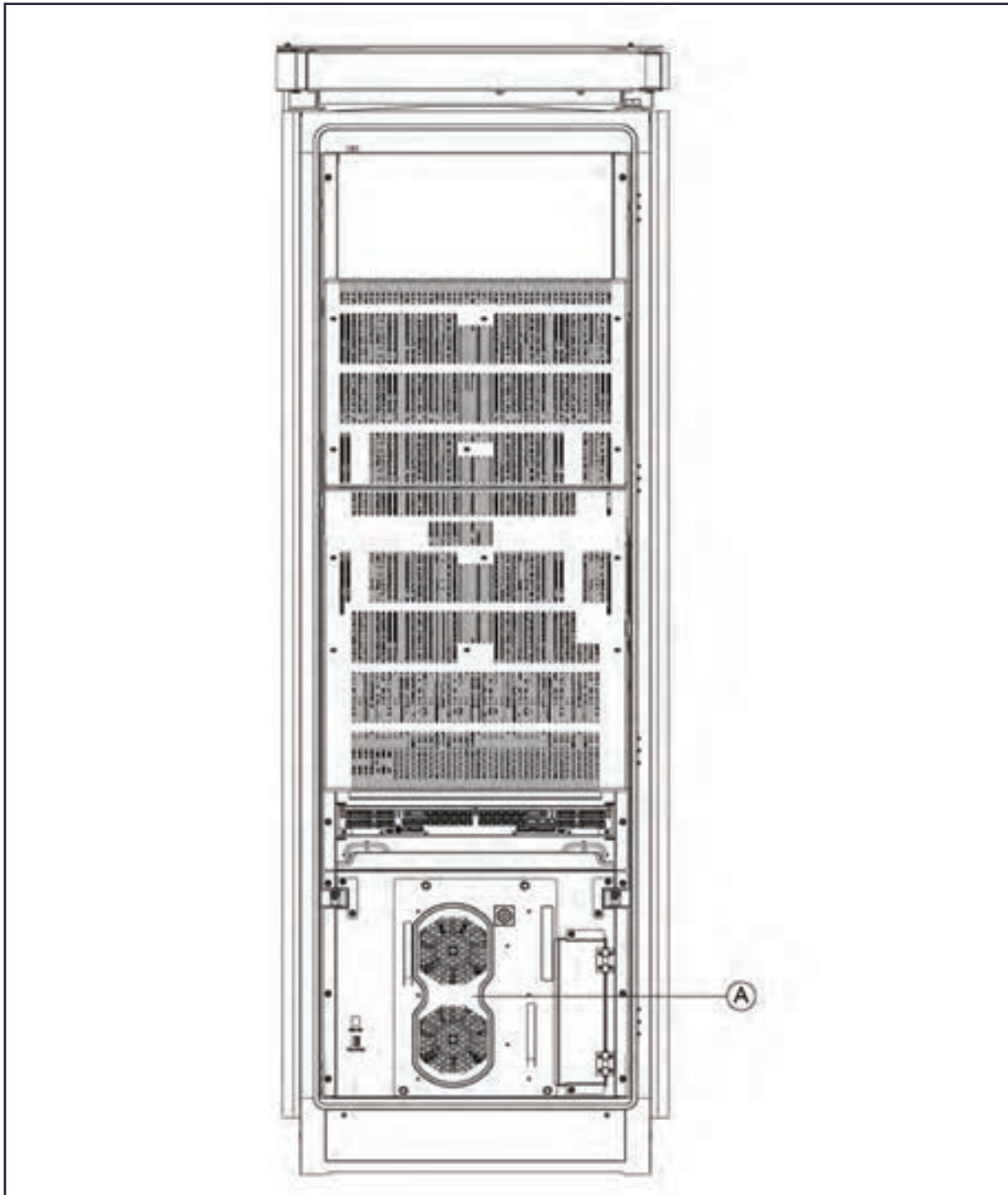
Figure 3-16 Position of the Cooling Unit
