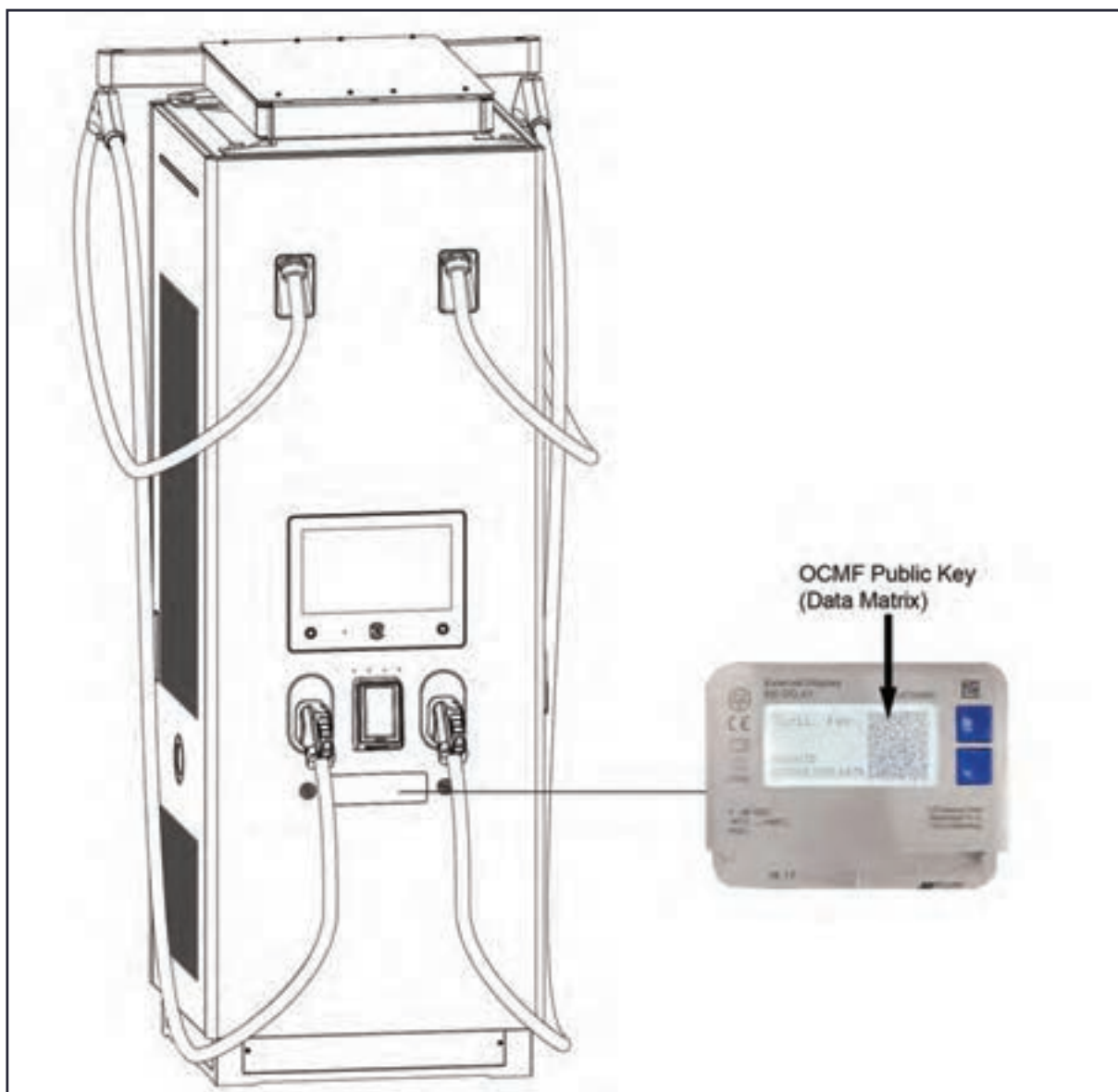
Figure 6-37 Location of the Public Key
