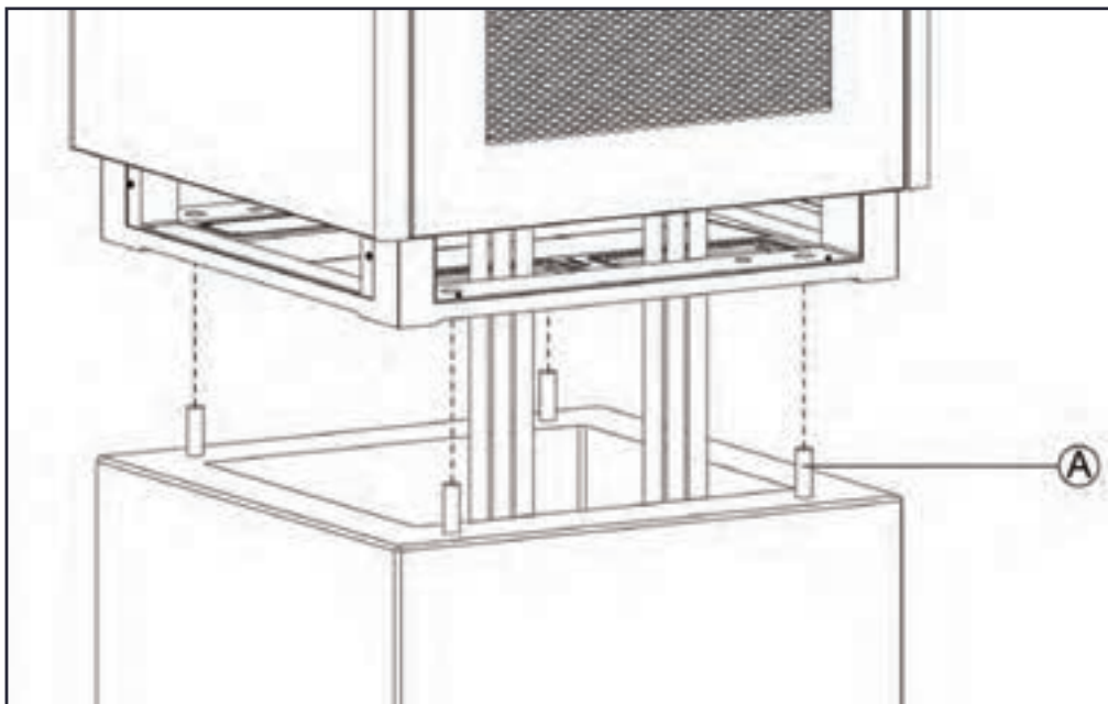
Figure 5-5 Lowering the Cabinet
