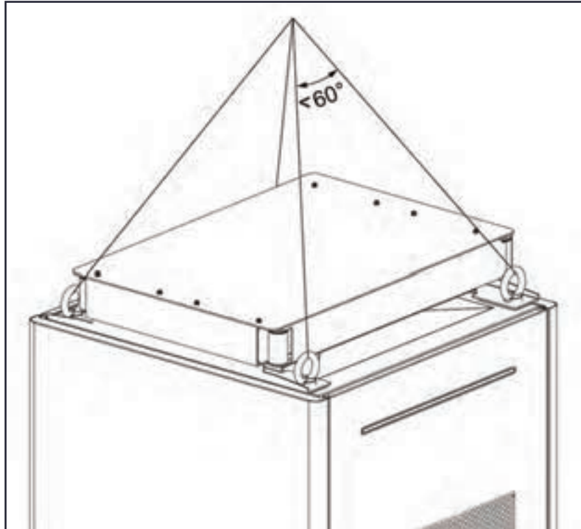
Figure 5-13 Hoisting the Cabinet
