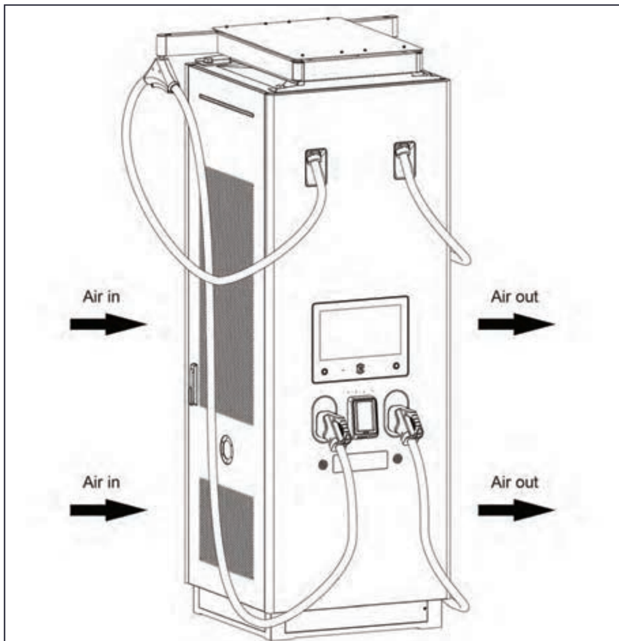
Figure 3-11 Direction of Airflow
