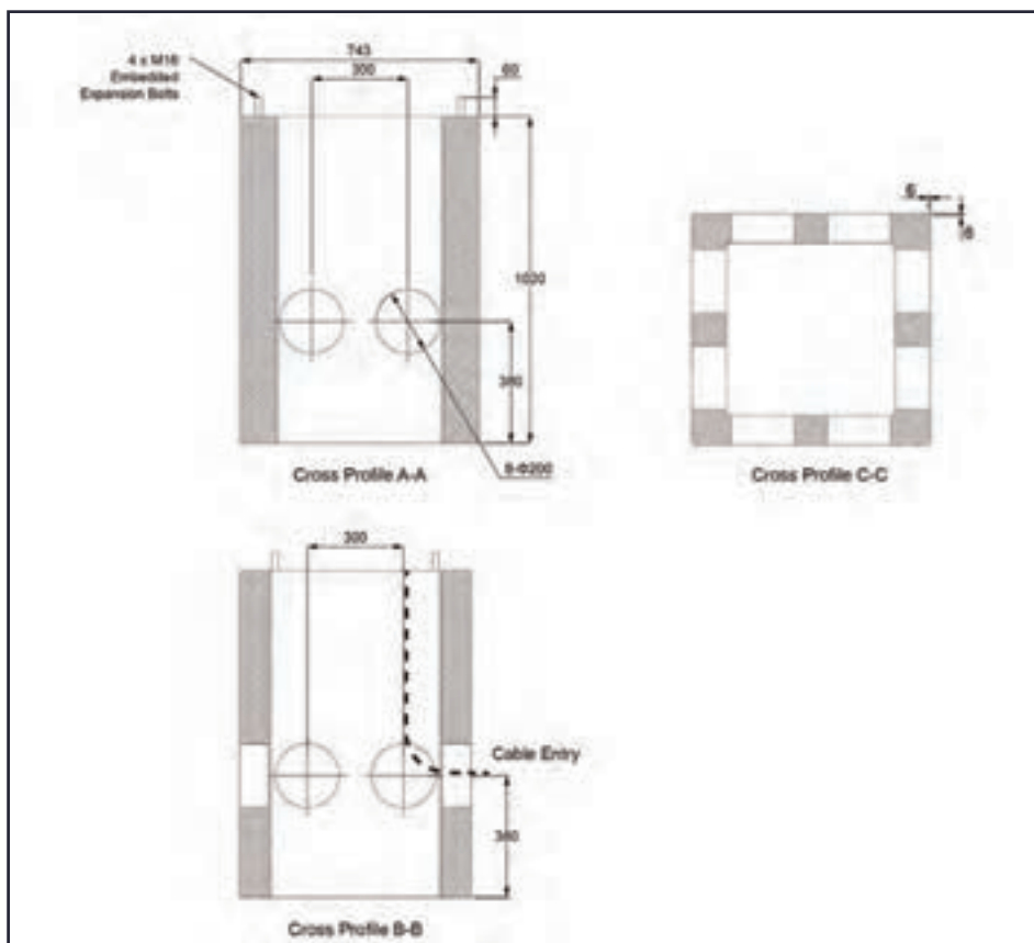
Figure 4-38 Foundation Dimensions
