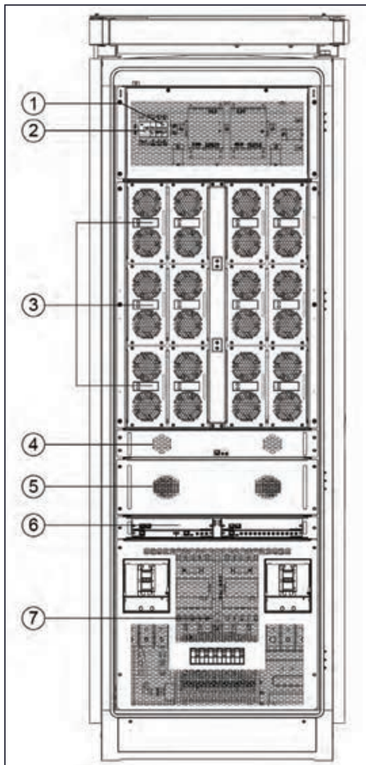
Figure 3-4 Product Overview (Inside)
