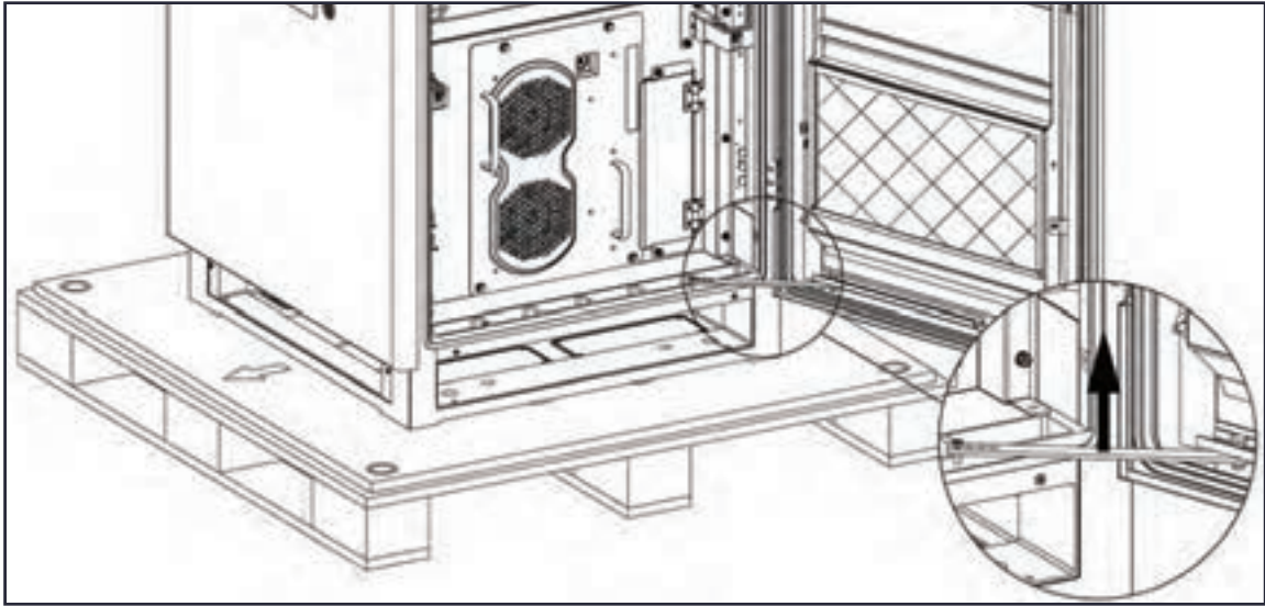
Figure 5-4 Lifting the Limit Linkage
