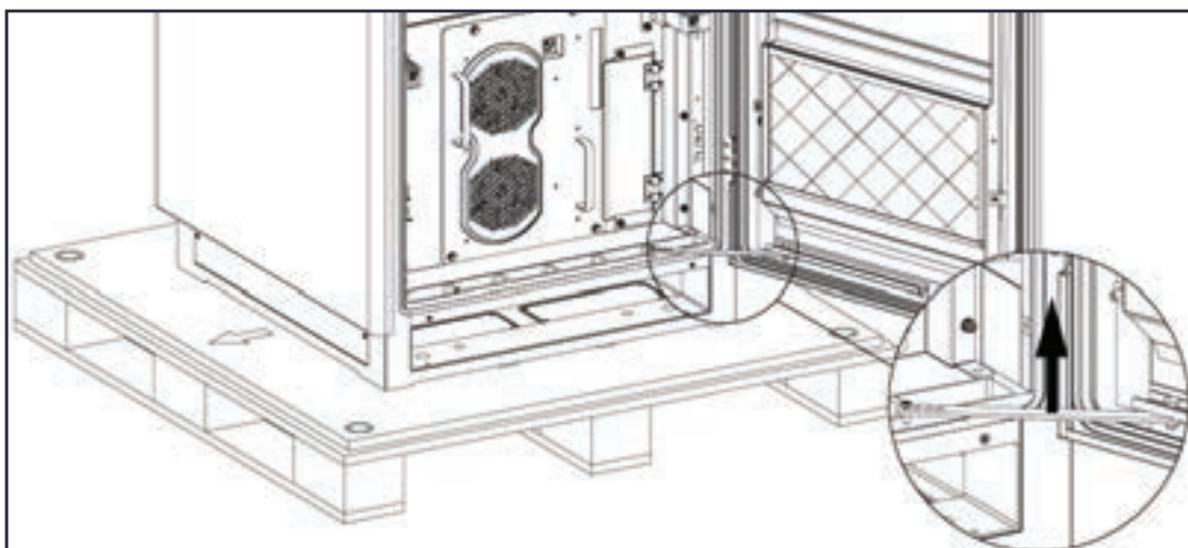
Figure 5-10 Lifting the Limit Linkage
