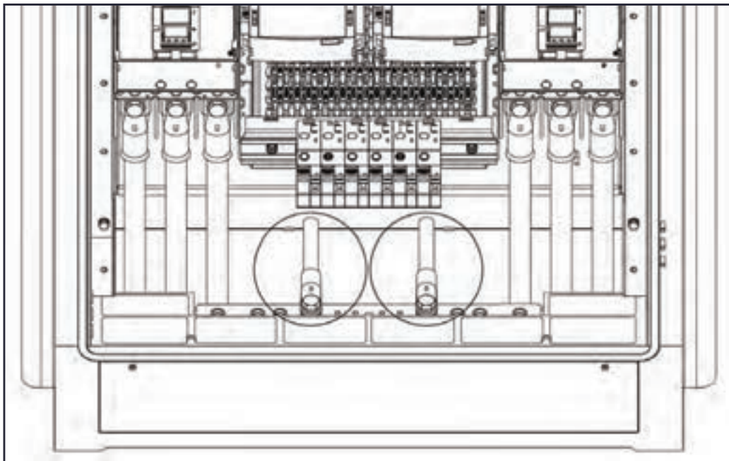
Figure 5-18 Connecting the PE Cable
