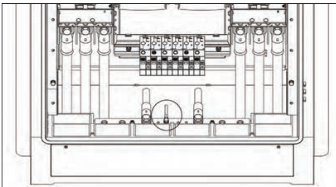
Figure 5-19 Connecting the Enclosure to the Earth
