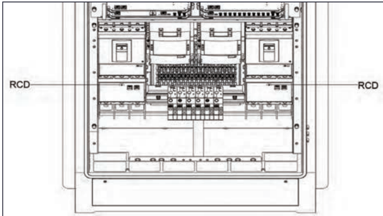
Figure 3-18 Position of the Additional RCDs in the Charging Station
