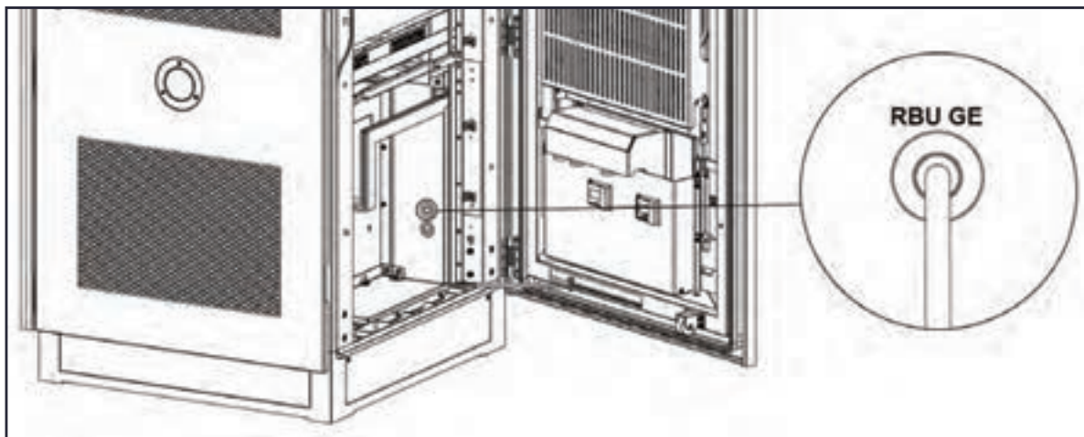
Figure 5-21 Connecting the Ethernet Cable
