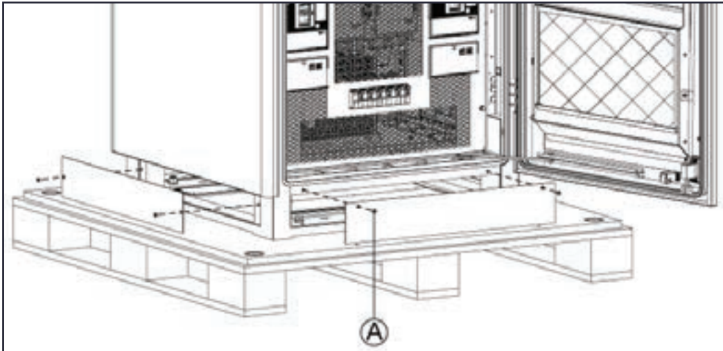
Figure 5-2 Removing the Base Covers
