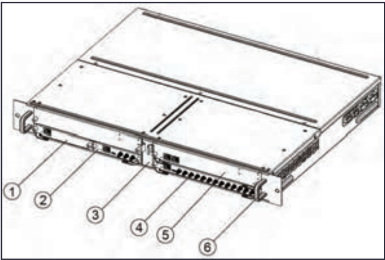
Figure 3-7 Control Module
