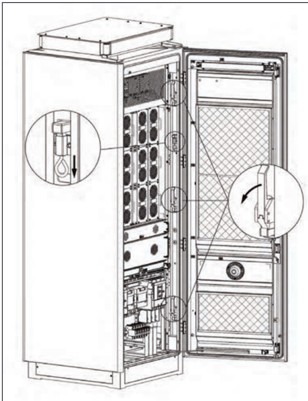
Figure 5-20 Opening the Front Door
