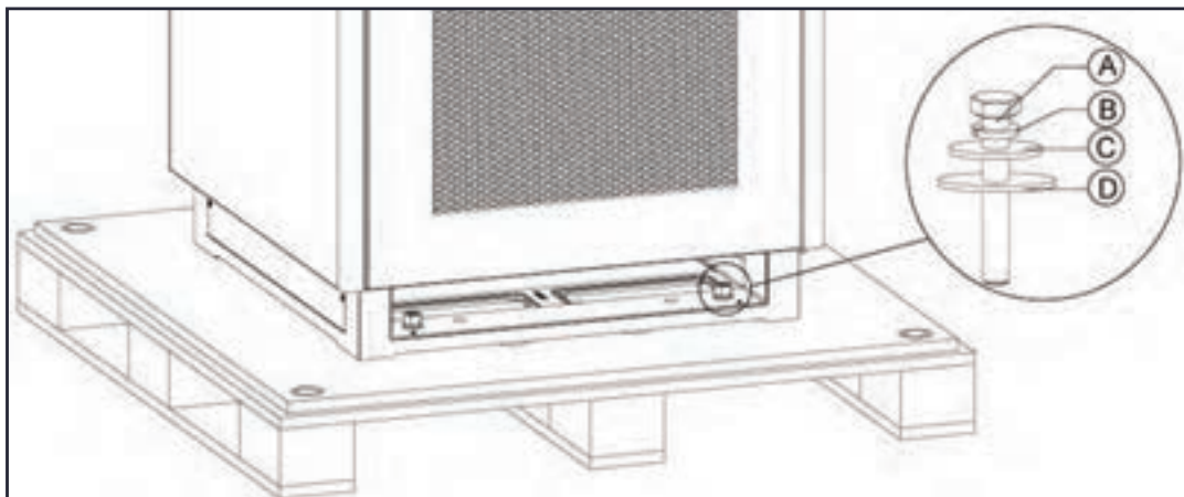
Figure 5-9 Removing from the Pallet
