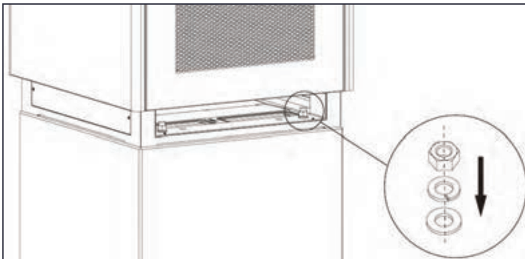
Figure 5-15 Securing the Cabinet onto Foundation
